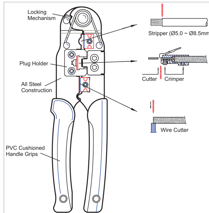
(Schematic Diagram)
